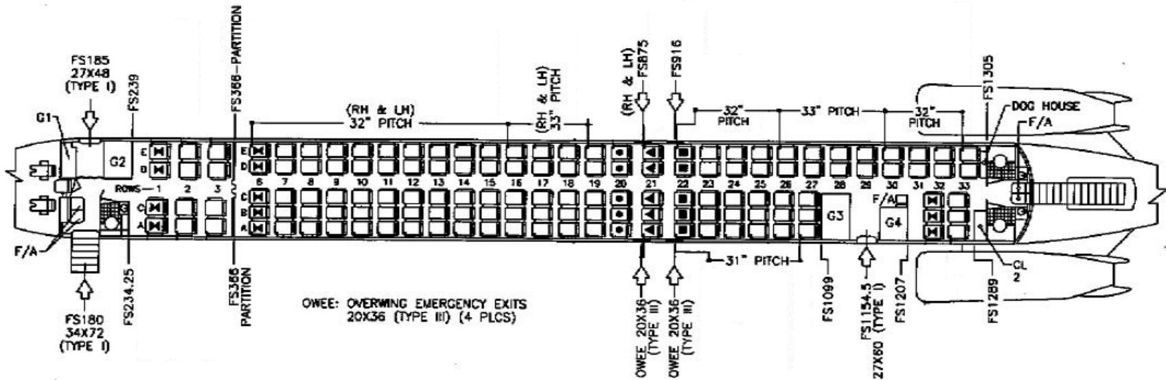
MD -83 / CABIN CONFIGURATION FOR 140 PAXS (12 FIRST CLASS - 128 TOURIST CLASS) VIEW LOOKING DOWN DETAIL A
